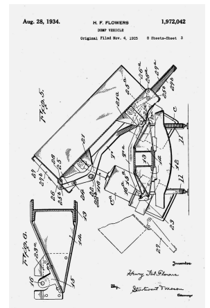
Patent application drawing for the dump vehicle, filed by H. Fort Flowers in 1931
